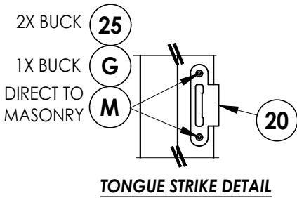
TONGUE STRIKE DETAIL
