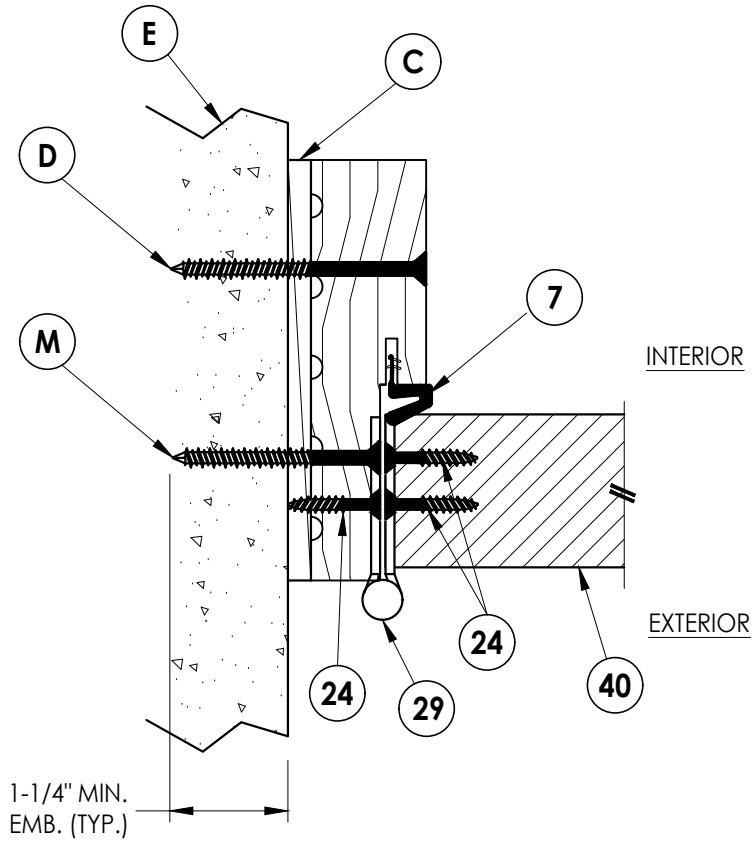
1 6 HORIZONTAL CROSS SECTION Shown Direct to Masonry Outswing only
