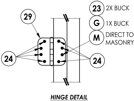
HINGE DETAIL
